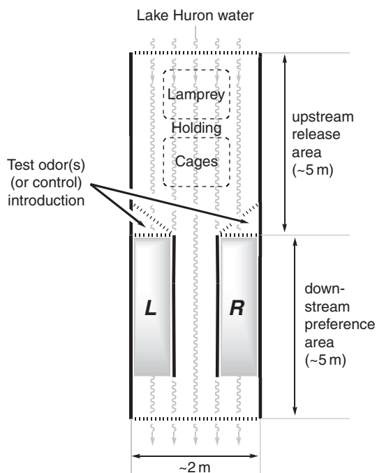
Figure 1 Schematic of the behavior maze used to guide isolation and identification of the sea lamprey pheromone. 19,27,28 Lake water mixed with a small amount of nonlamprey river water flows slowly from top to bottom at a depth of c. 10 cm in this two-choice maze, where preference of adult lamprey is assessed by measuring the ratio of time in the right channel to time in the left ( t_R/t_L ), while odor is into one side or the other.
