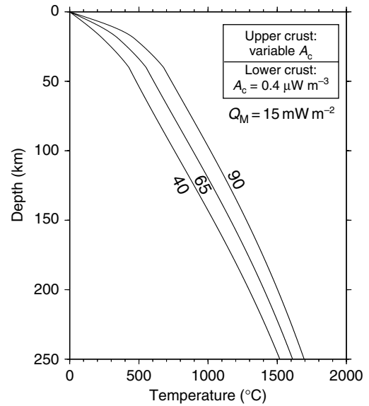
Figure 10 Three continental geotherms calculated for surface heat flux = 40, 65, and 90 \text{mW m}^{-2} . Calculations are made with temperature-dependent conductivity (see Appendix) and for the same Moho heat flow of 15 \text{mW m}^{-2} . Crustal heat production is assumed to be distributed in two layers of equal thickness with a fixed value of 0.4 \mu\text{W m}^{-3} for heat production in the lower crust. With such models, changing the surface heat flux by 25 \text{mW m}^{-2} leads to changes of \approx 110^\circ\text{C} and 100^\circ\text{C} for temperatures at the Moho and at 200 km depth.
