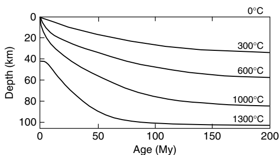
Figure 9 Isotherms in the oceanic lithosphere from the plate model of McKenzie et al. (2005). Earthquake hypocenters are confined to shallow regions above the 600°C isotherm.
