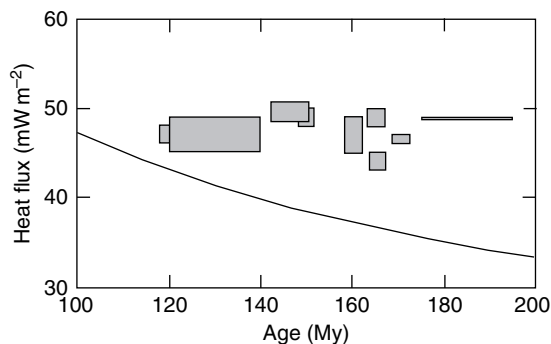
Figure 7 Closeup of the reliable oceanic heat flux data through sea floor older than 100 My. Within measurement uncertainty, these data suggest that heat flux is constant and about 48 \text{ mW m}^{-2} . Reproduced from Lister CRB, Sclater JG, Nagihara S, Davis EE, and Villinger H (1990) Heat flow maintained in ocean basins of great age – Investigations in the north-equatorial West Pacific. Geophysical Journal International 102: 603–630.
